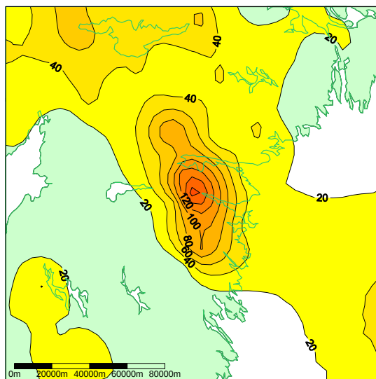
Figur 52. Nederbördssumma[mm] 1973-07-08 – 1973-07-09.
