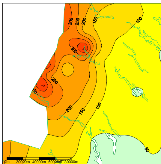
Figur 122. Nederbördssumma [mm] 1989-01-08 – 1989-02-06.
