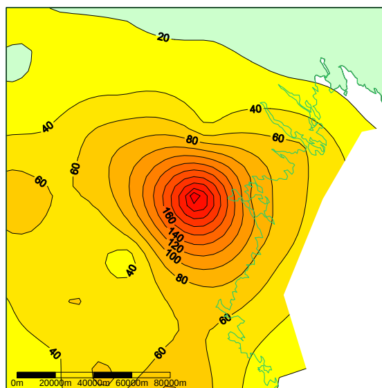
Figur 82. Nederbördssumma [mm] 1997-07-27 – 1997-08-02.
