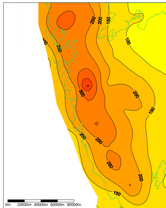
Figur 126. Nederbördssumma[mm] 2006-11-15 – 2006-12-14.
