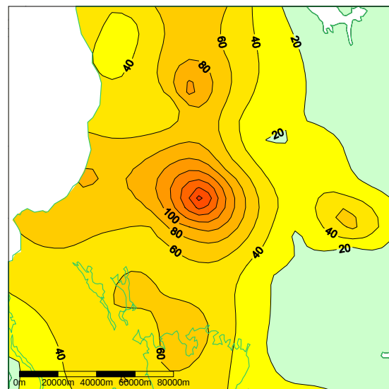
Figur 68. Nederbördssumma [mm] 2004-08-01 – 2004-08-04.
