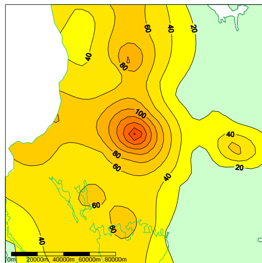
Figur 50. Nederbördssumma [mm] 2004-08-03 – 2004-08-04.
